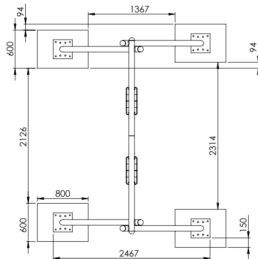
Diagram 3: Top view with dimension details „vola2“
