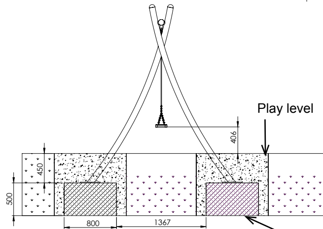
Diagram 2: Side view with dimension details „vola1“
