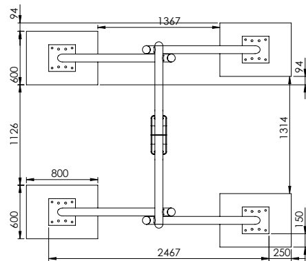
Diagram 3: Top view with dimension details „vola1“
