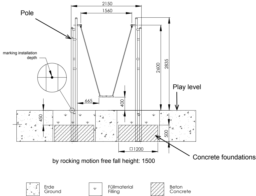
Diagram 2: Side view with dimension details „statuo“
