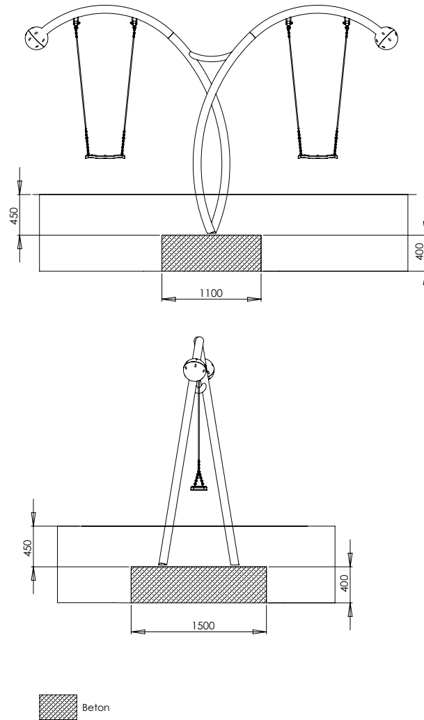
Diagram 2: Side view with dimension details
