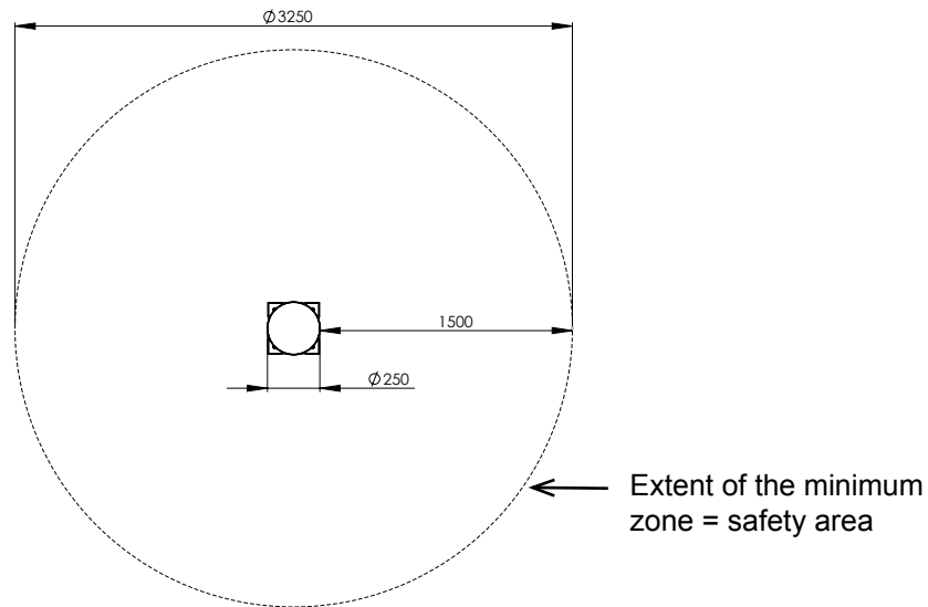
Diagram 3: Top view „rotundo5“
