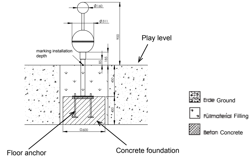
Diagram 2: Side view with dimension details „rotundo2“
