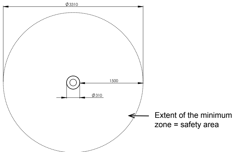
Diagram 3: Top view „rotundo2“
