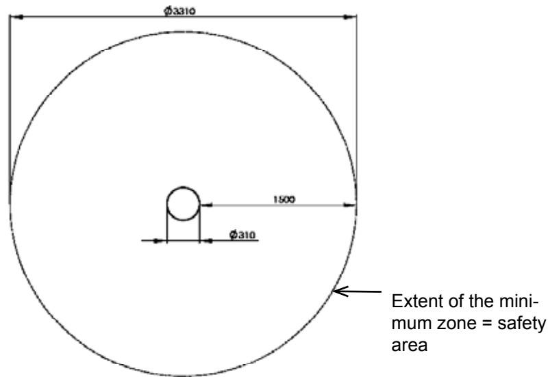
Diagram 3: Top view „rotundo1“
