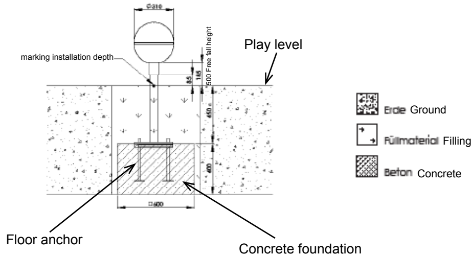
Diagram 2: Side view with dimension details „rotundo1“
