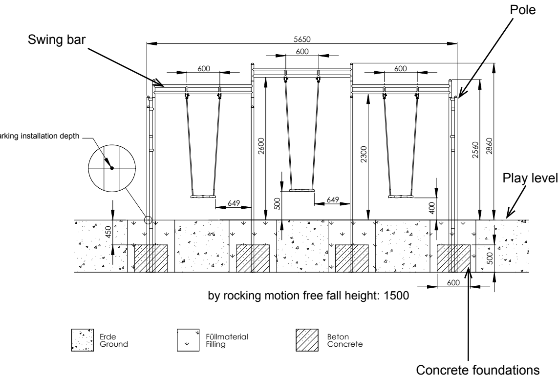
Diagram 2: Side view with dimension details „patis3“
