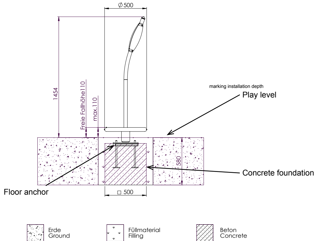
Diagram 2: Side view with dimension details „cita“
