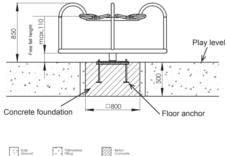
Diagram 2: Side view with dimension details „circulus4“
