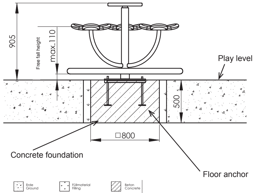
Diagram 2: Side view with dimension details „circulus3“
