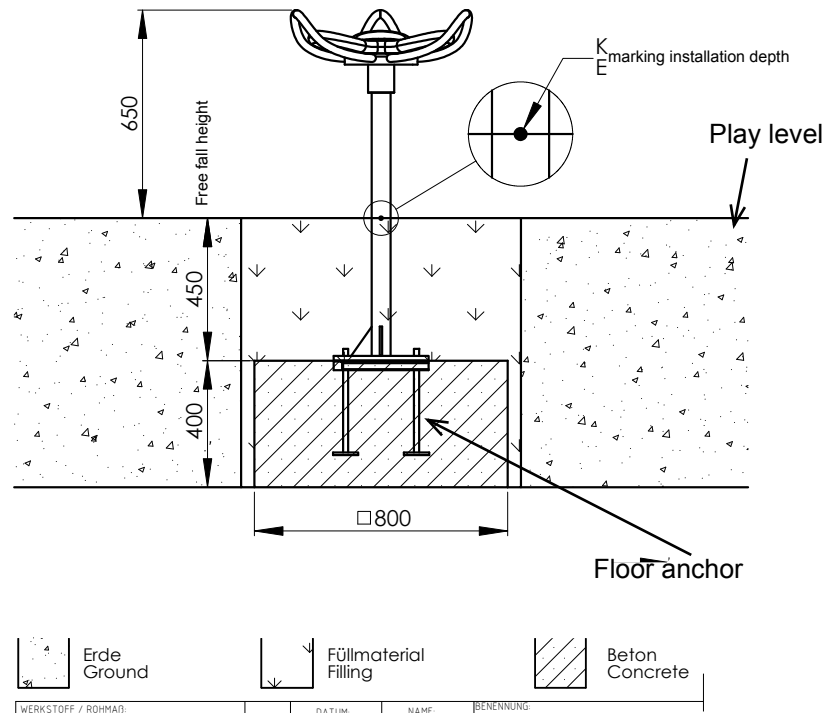
Diagram 2: Side view with dimension details „circulus1“
