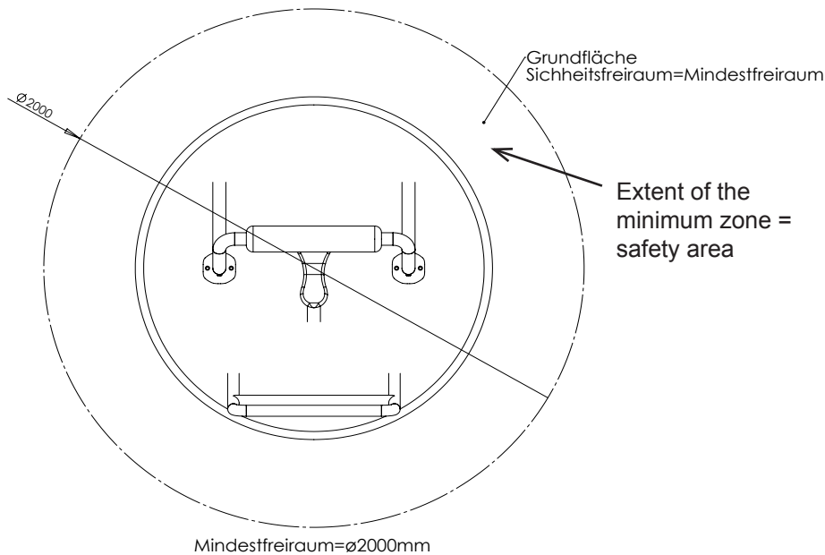
Diagram 3: Top view „Back trainer“
