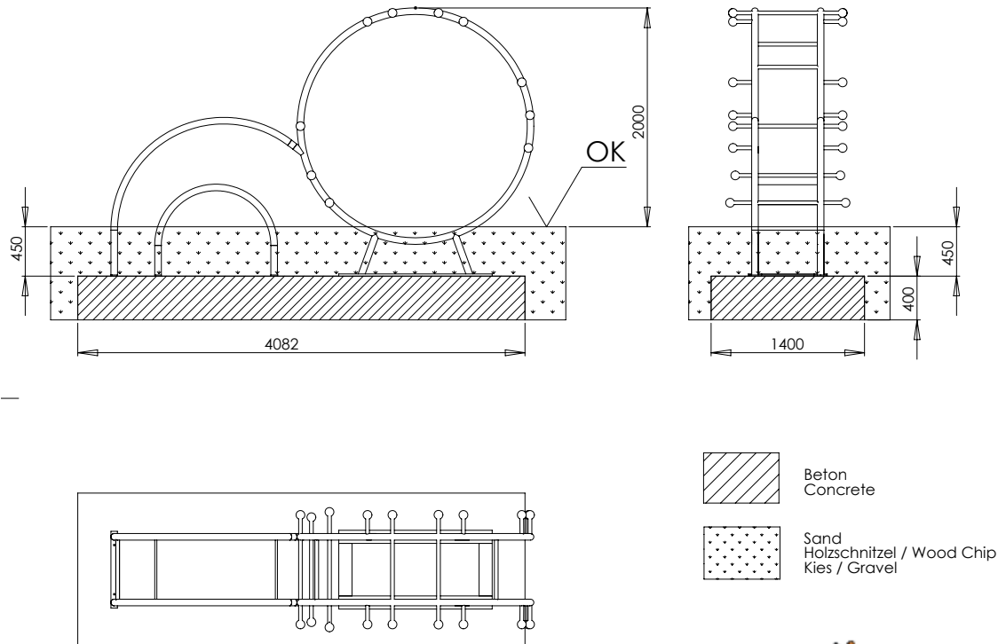
Diagram 2: Side view with dimension details „Multi-functional trainer“
