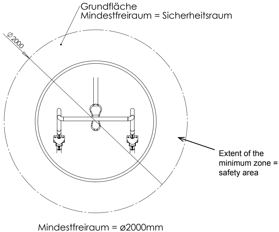
Diagram 3: Top view „Power bench, sitting“
