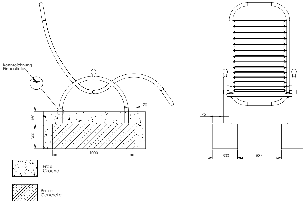
Diagram 1: Foundation
