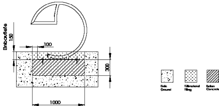
Diagram 2: Side view with dimension details „unio2“
