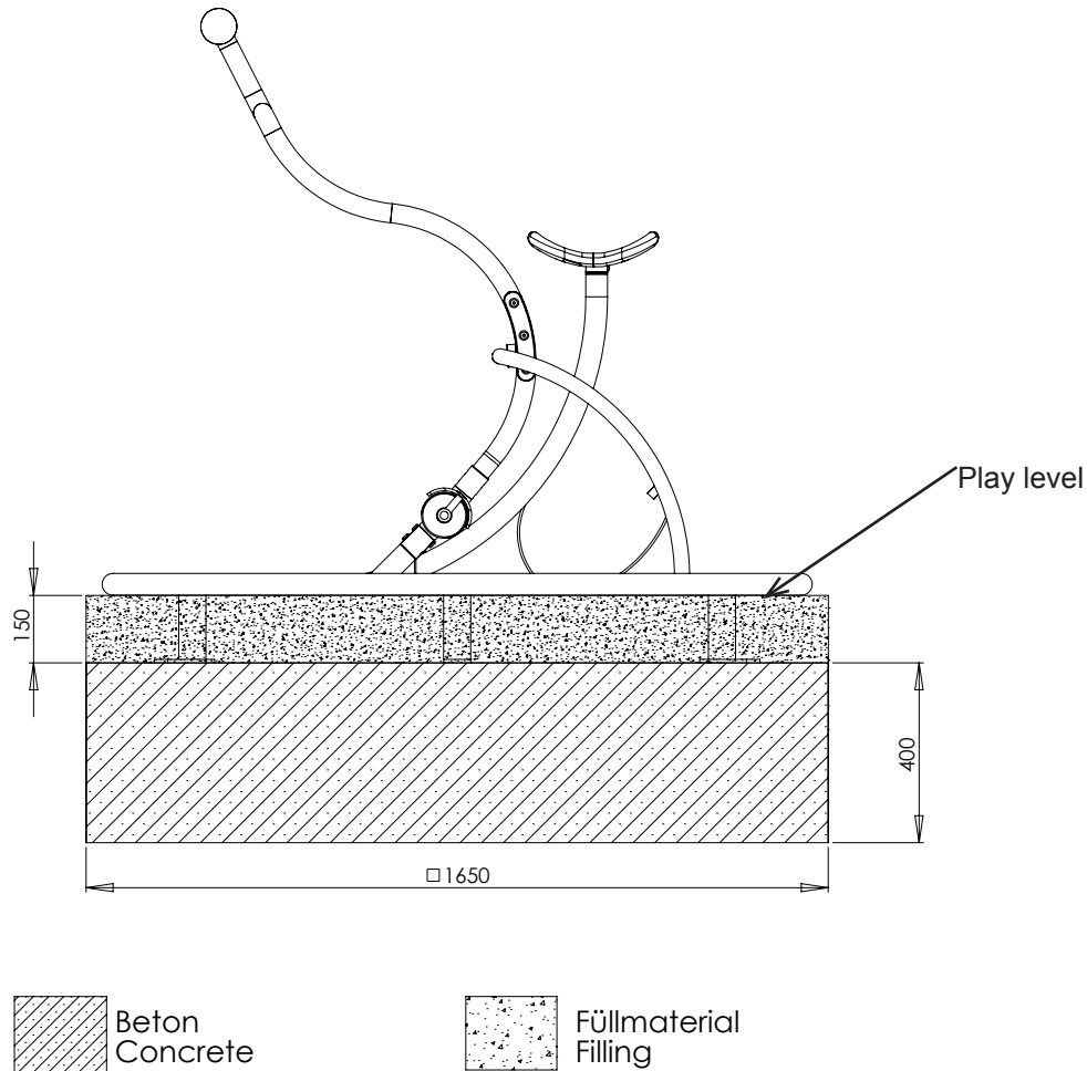
Diagram 2: Side view with dimension details „Rudder trainer“
