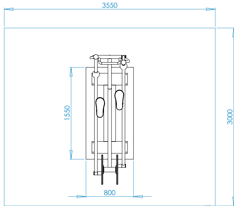
Diagram 3: Top view „Crosstrainer Stepper“
