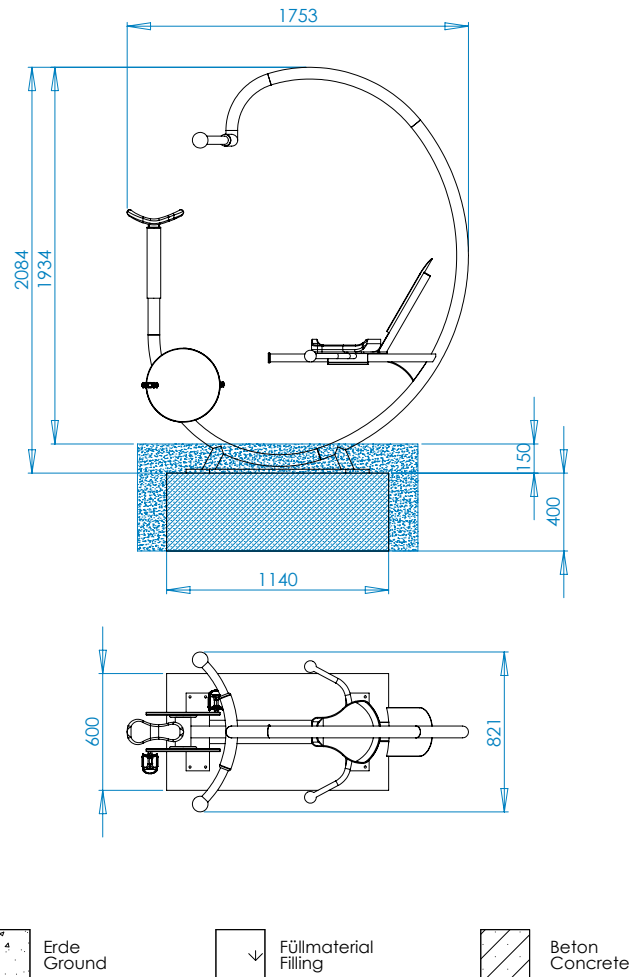
Diagram 2: Side view with dimension details „Fitness bike“
