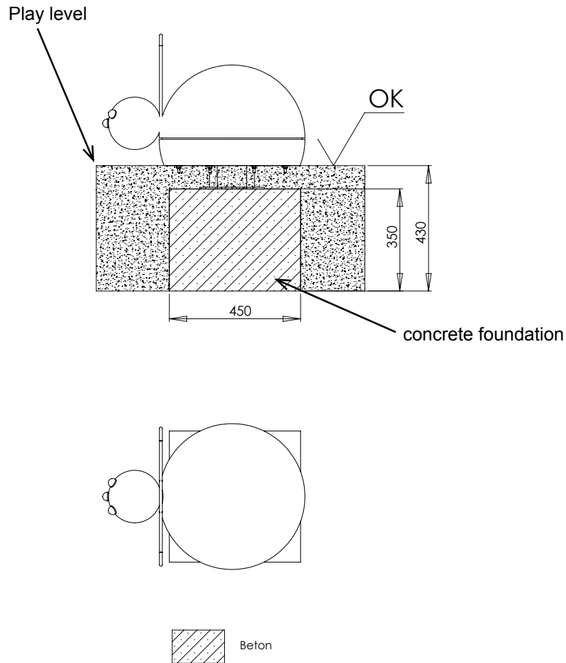
Diagram 2: Side view with dimension details „Lana“
