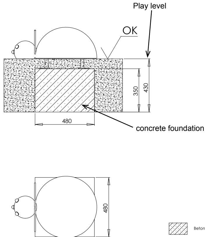
Diagram 2: Side view with dimension details „Lilly“
