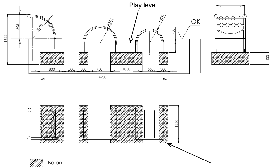
Diagram 2: Side view with dimension details „Erika“
