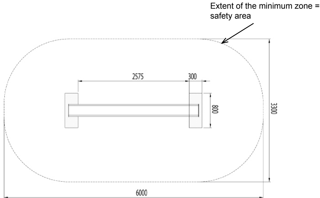
Diagram 3: Top view
