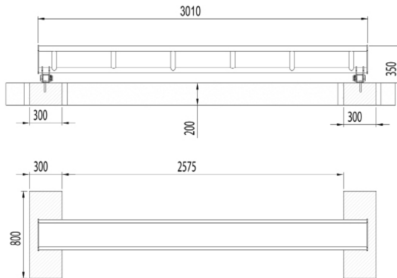
Diagram 2: Side view with dimension details „librium“
