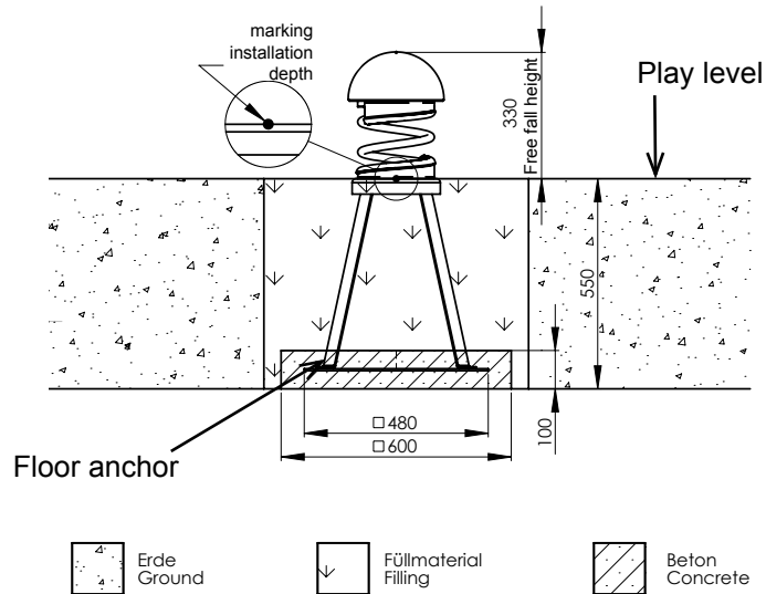
Diagram 2: Side view with dimension details „pinna2“
