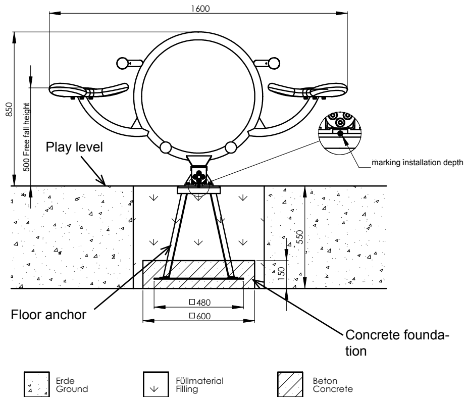
Diagram 2: Side view with dimension details „altus2“
