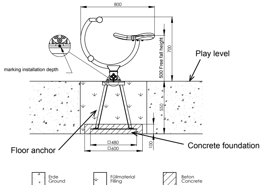
Diagram 2: Side view with dimension details „altus1“
