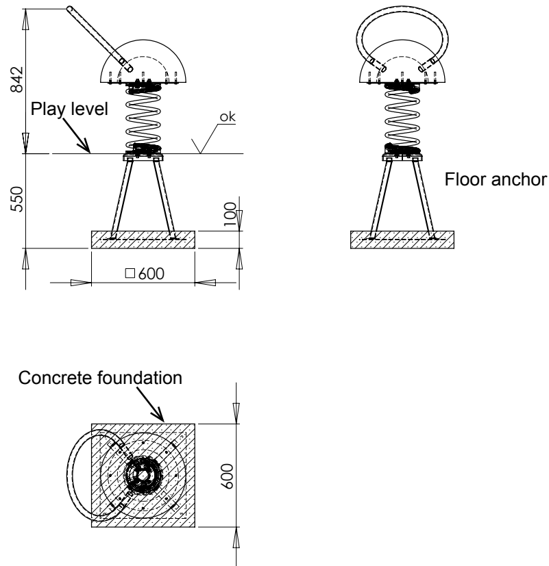
Diagram 2: Side view with dimension details „caligo pluma 2014“
