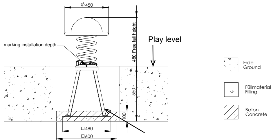
Diagram 2: Side view with dimension details „pinna“
