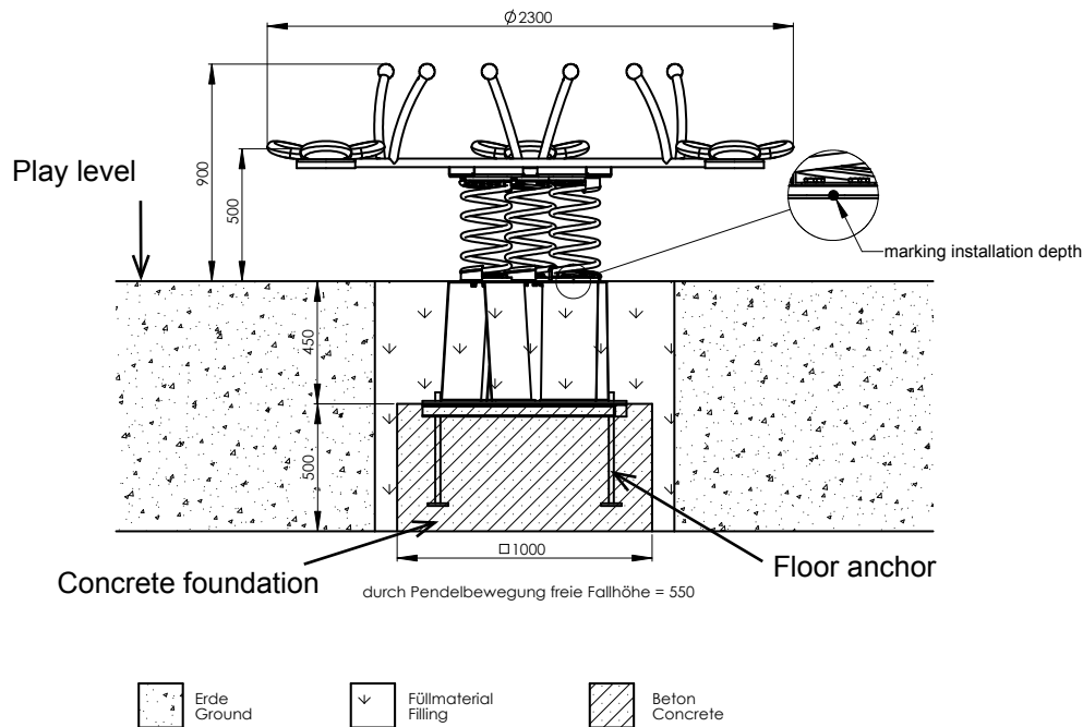
Diagram 2: Side view with dimension details „papilio3“
