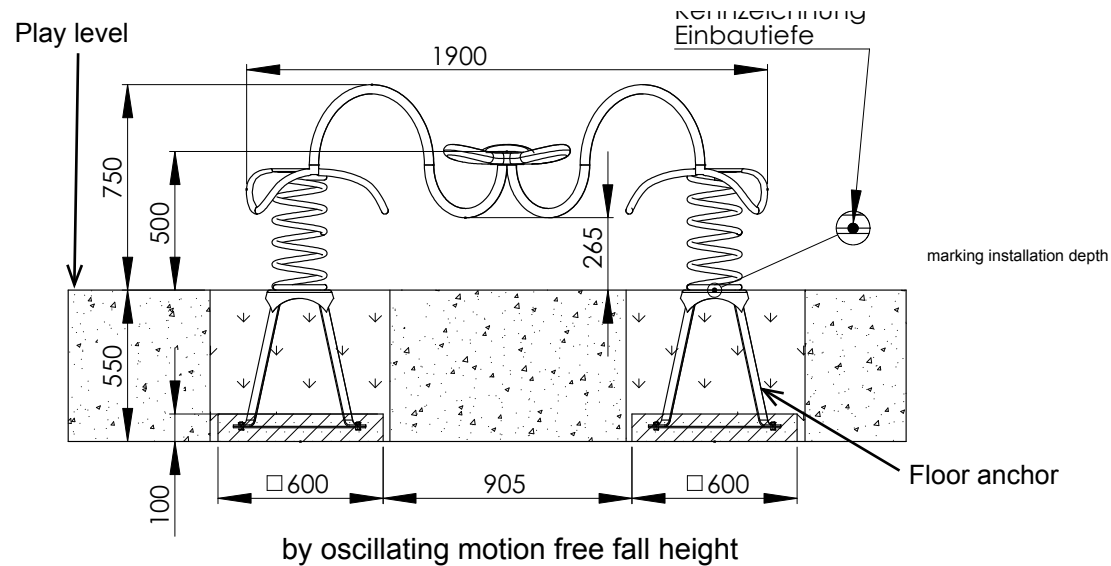
Diagram 2: Side view with dimension details „frondis2“
