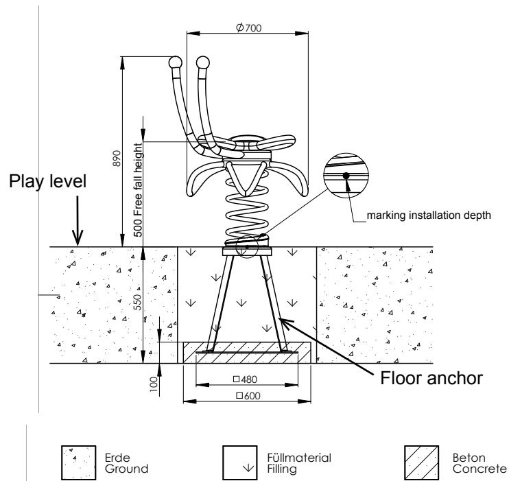
Diagram 2: Side view with dimension details „papilio1“
