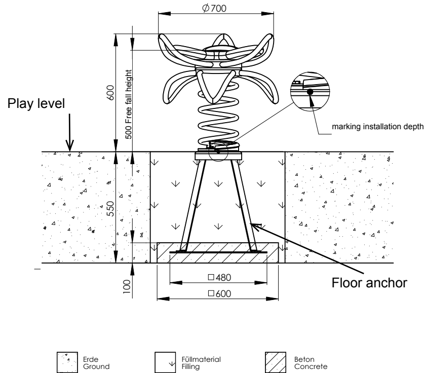
Diagram 2: Side view with dimension details „frondis1“
