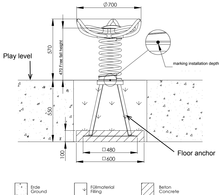
Diagram 2: Side view with dimension details „floris1“
